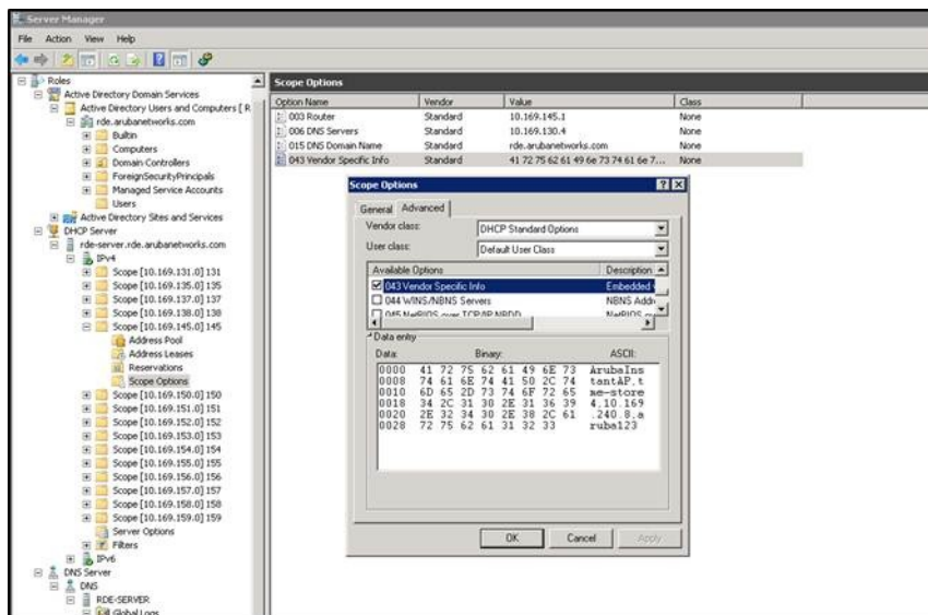
Figure 29 Vendor-Specific DHCP options
